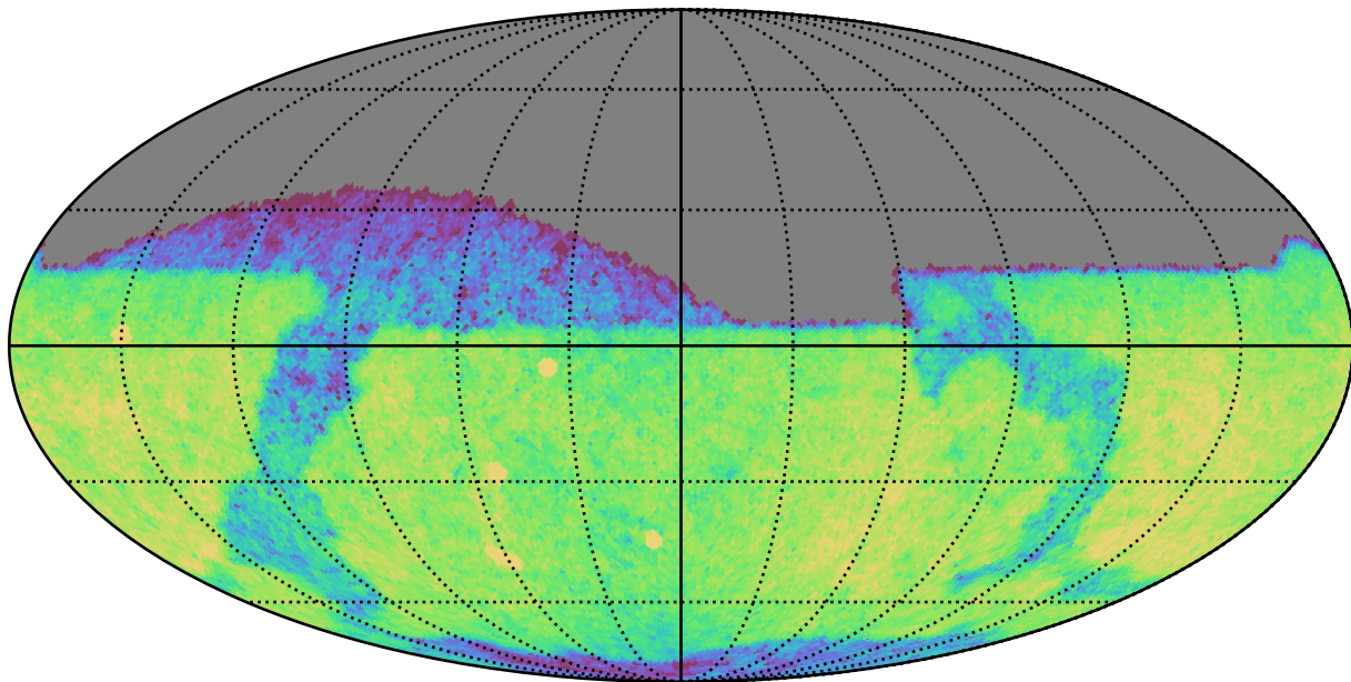
weather_cloudso35v3.4_10yrs Yr 1 z band: CoaddM5
