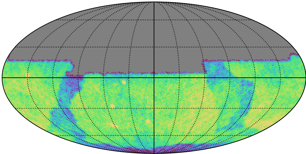
weather_cloudso35v3.4_10yrs Yr 1 y band: CoaddM5
