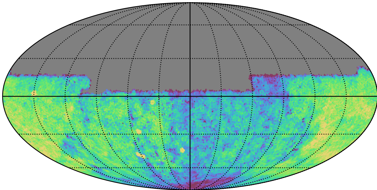
weather_cloudso35v3.4_10yrs Yr 1 u band: CoaddM5
