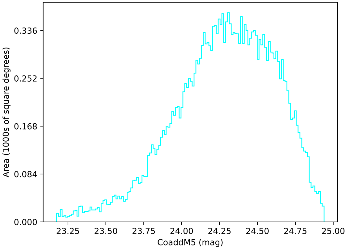
weather_cloudso35v3.4_10yrs Yr 1 u band: CoaddM5
