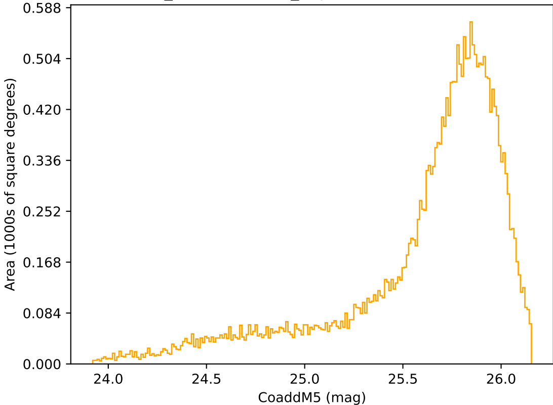
weather_cloudso35v3.4_10yrs Yr 1 r band: CoaddM5
