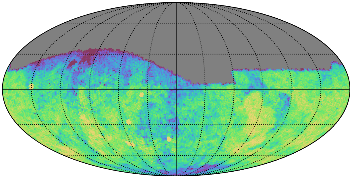
weather_cloudso35v3.4_10yrs Yr 1 g band: CoaddM5
