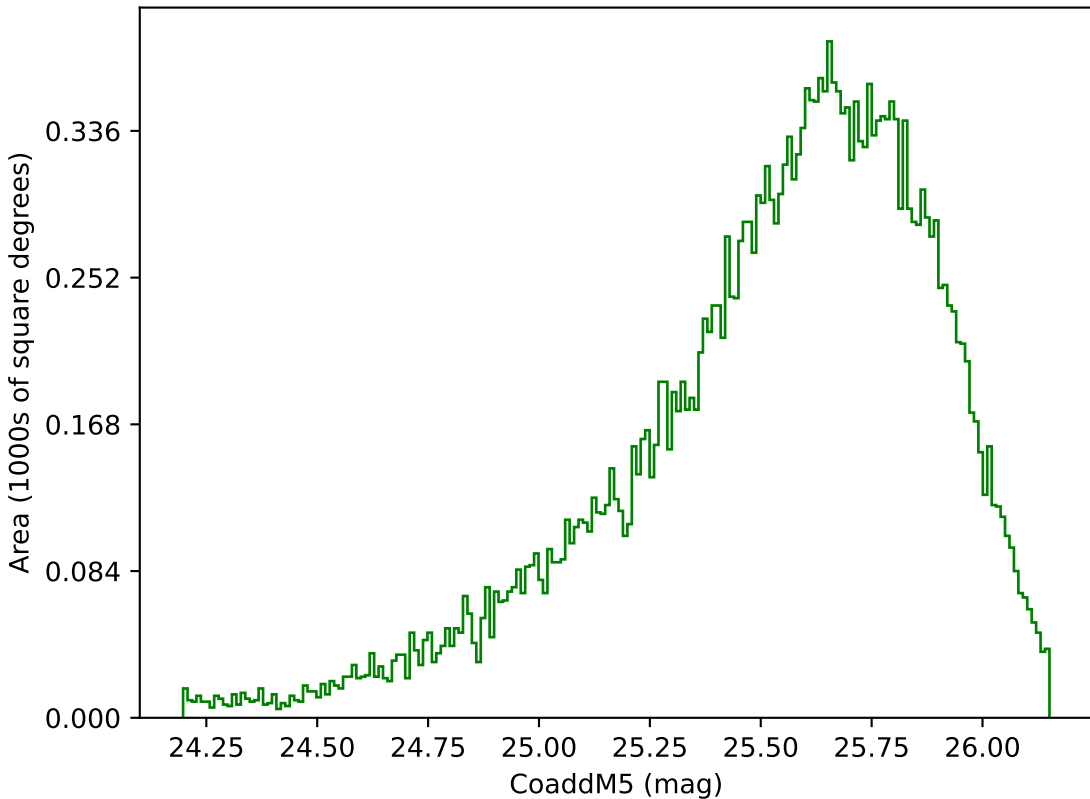
weather_cloudso35v3.4_10yrs Yr 1 g band: CoaddM5
