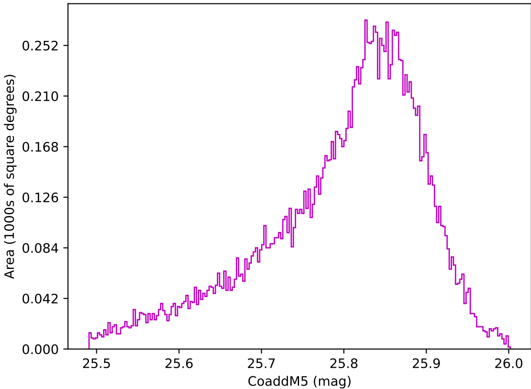
weather_cloudso35v3.4_10yrs WFD z band: CoaddM5
