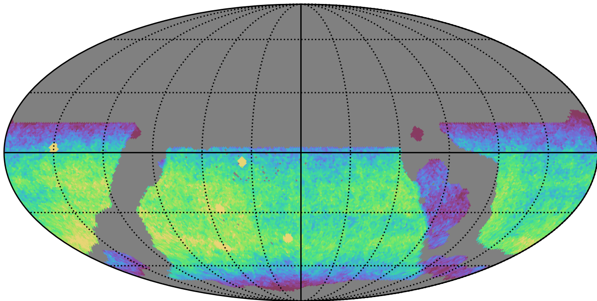
weather_cloudso35v3.4_10yrs WFD y band: CoaddM5
