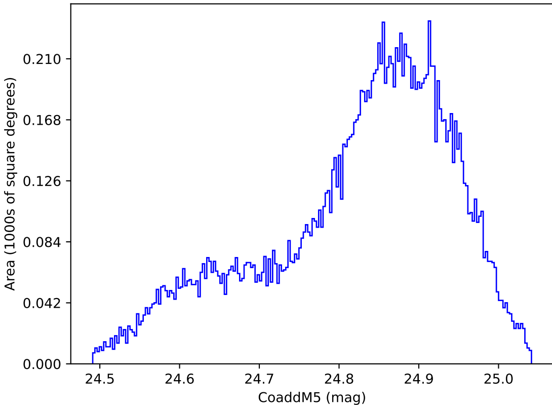
weather_cloudso35v3.4_10yrs WFD y band: CoaddM5
