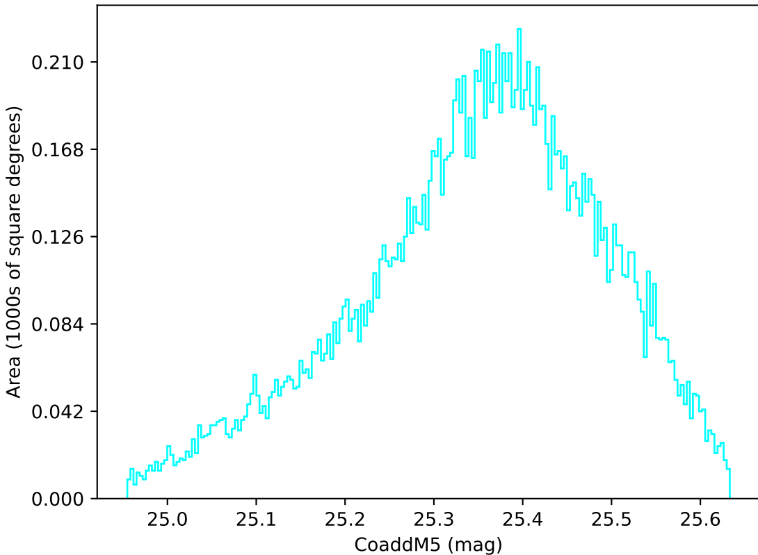
weather_cloudso35v3.4_10yrs WFD u band: CoaddM5
