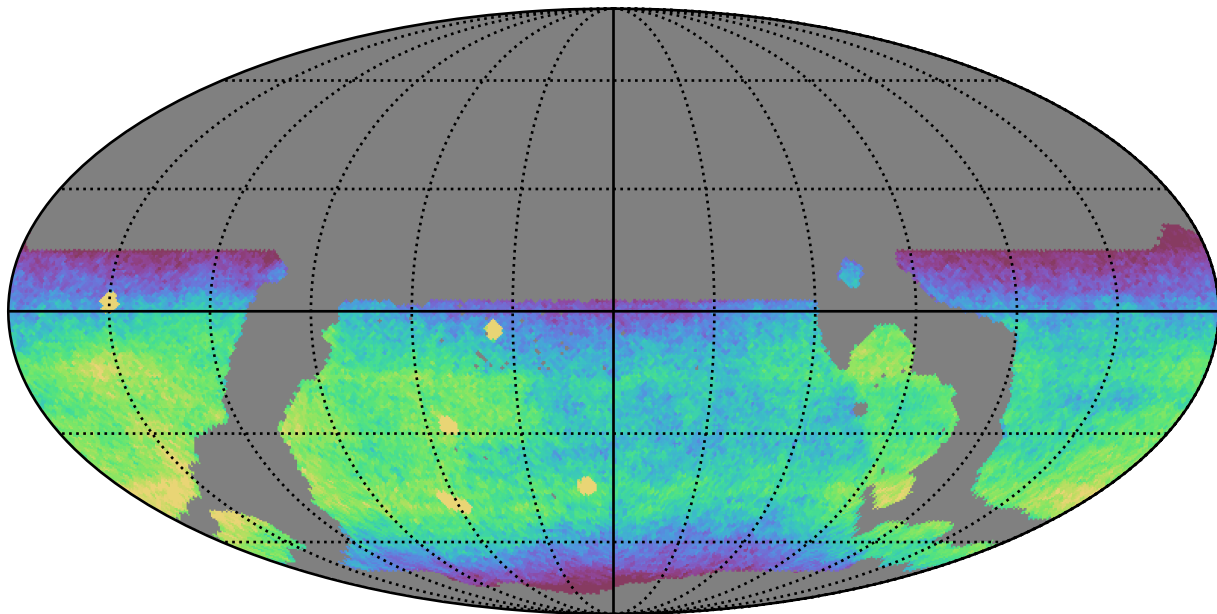
weather_cloudso35v3.4_10yrs WFD r band: CoaddM5
