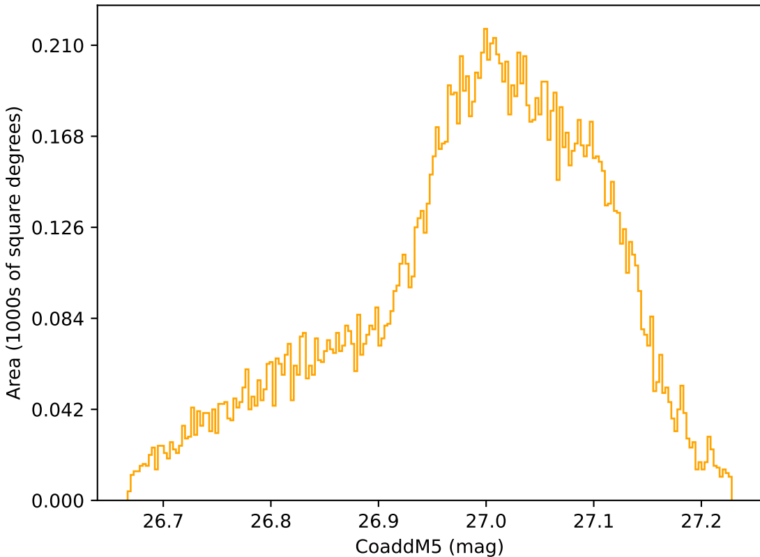
weather_cloudso35v3.4_10yrs WFD r band: CoaddM5
