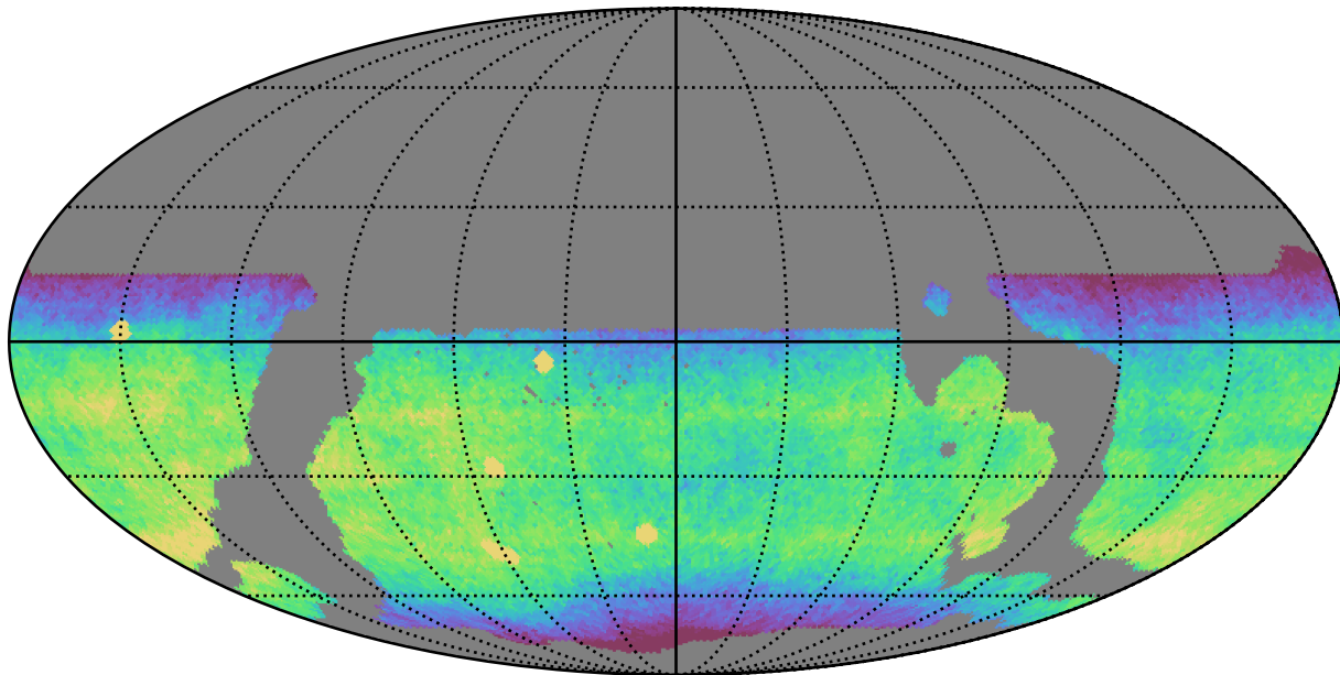
weather_cloudso35v3.4_10yrs WFD i band: CoaddM5
