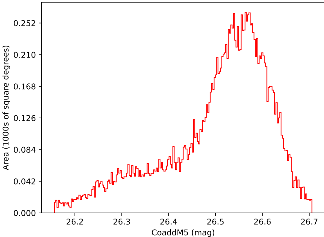
weather_cloudso35v3.4_10yrs WFD i band: CoaddM5
