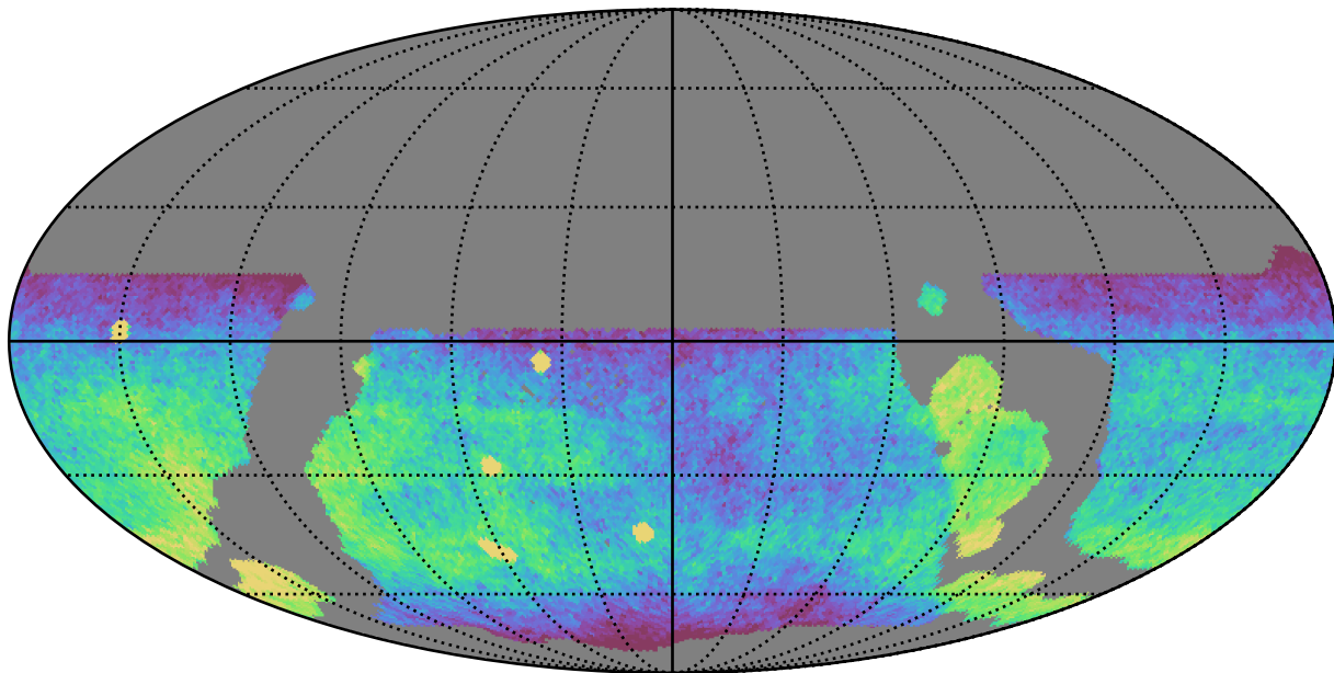
weather_cloudso35v3.4_10yrs WFD g band: CoaddM5
