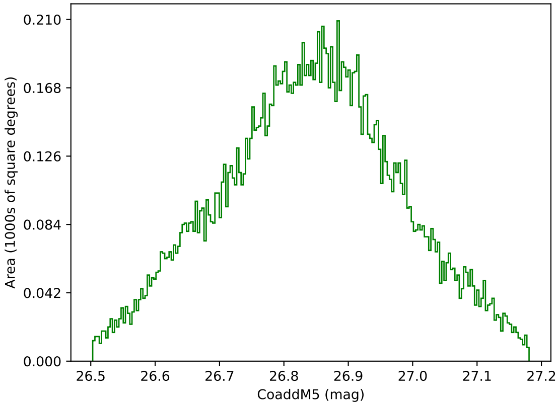
weather_cloudso35v3.4_10yrs WFD g band: CoaddM5
