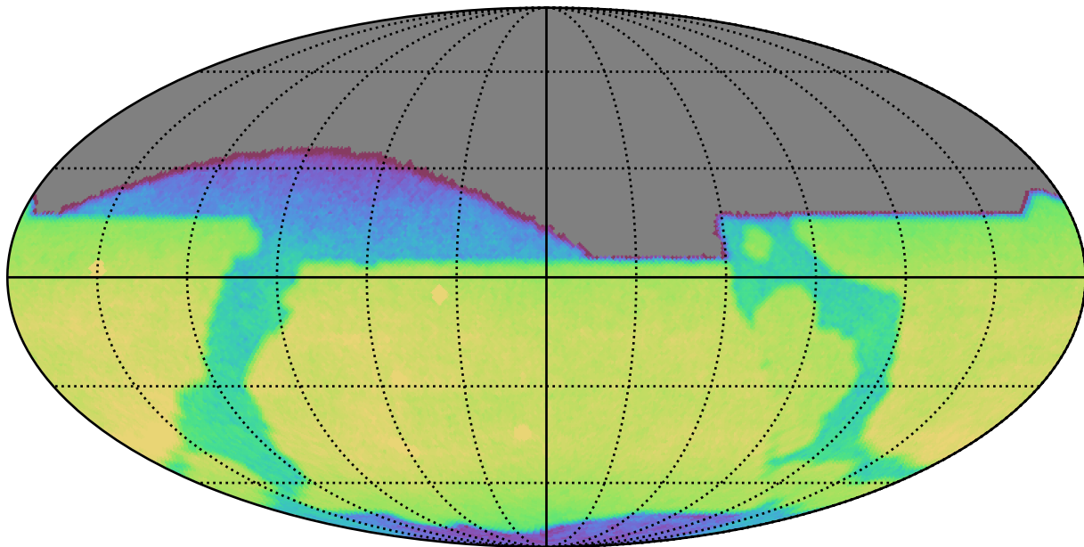
weather_cloudso35v3.4_10yrs All sky z band: CoaddM5
