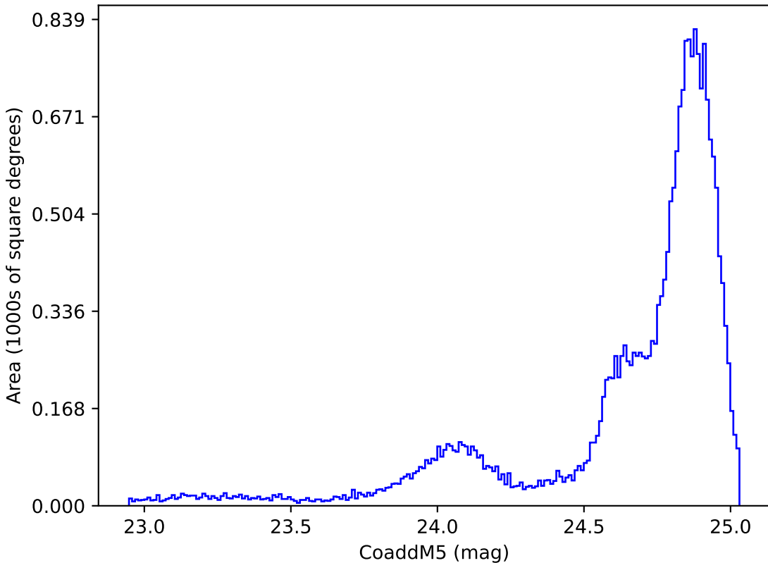
weather_cloudso35v3.4_10yrs All sky y band: CoaddM5
