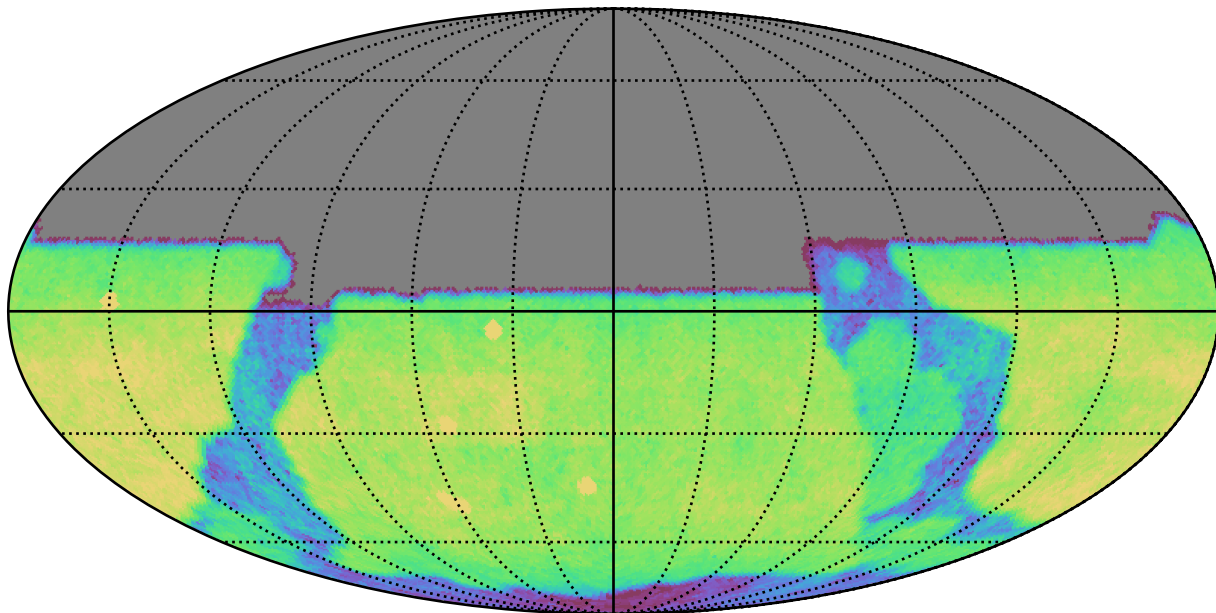
weather_cloudso35v3.4_10yrs All sky u band: CoaddM5
