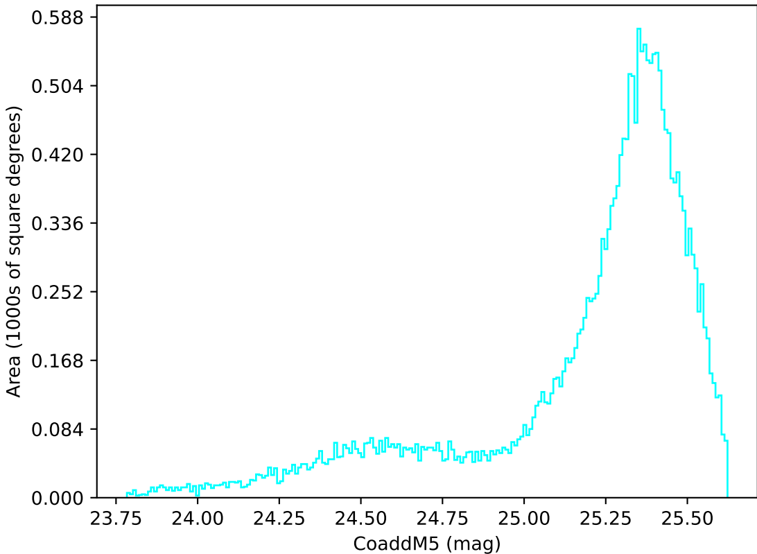
weather_cloudso35v3.4_10yrs All sky u band: CoaddM5
