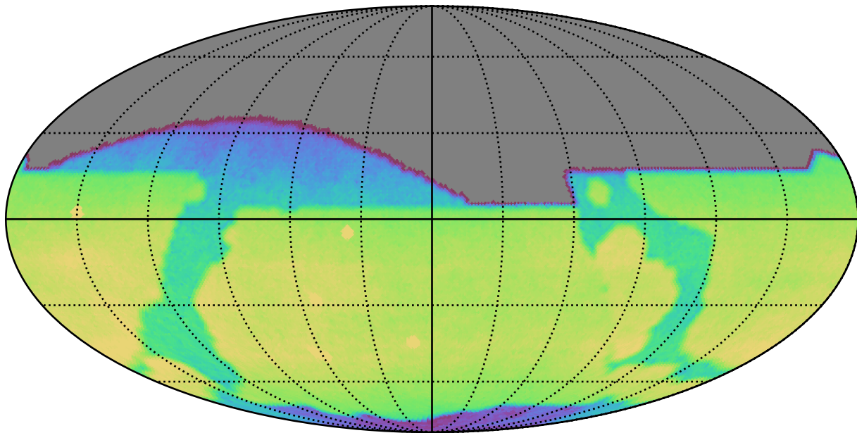
weather_cloudso35v3.4_10yrs All sky r band: CoaddM5
