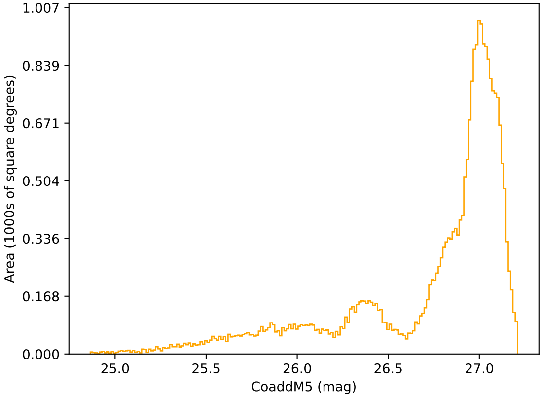
weather_cloudso35v3.4_10yrs All sky r band: CoaddM5
