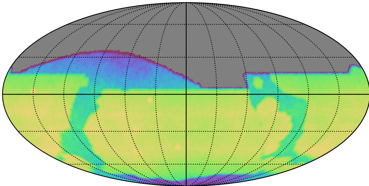
weather_cloudso35v3.4_10yrs All sky i band: CoaddM5
