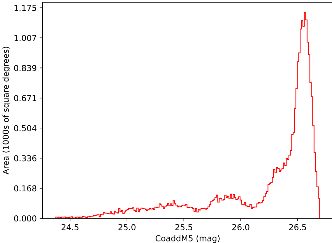
weather_cloudso35v3.4_10yrs All sky i band: CoaddM5
