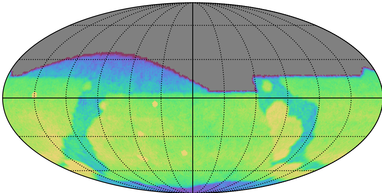
weather_cloudso35v3.4_10yrs All sky g band: CoaddM5
