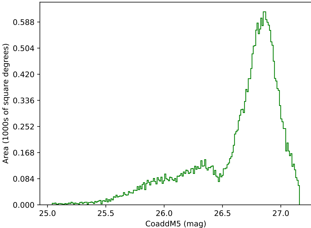
weather_cloudso35v3.4_10yrs All sky g band: CoaddM5
