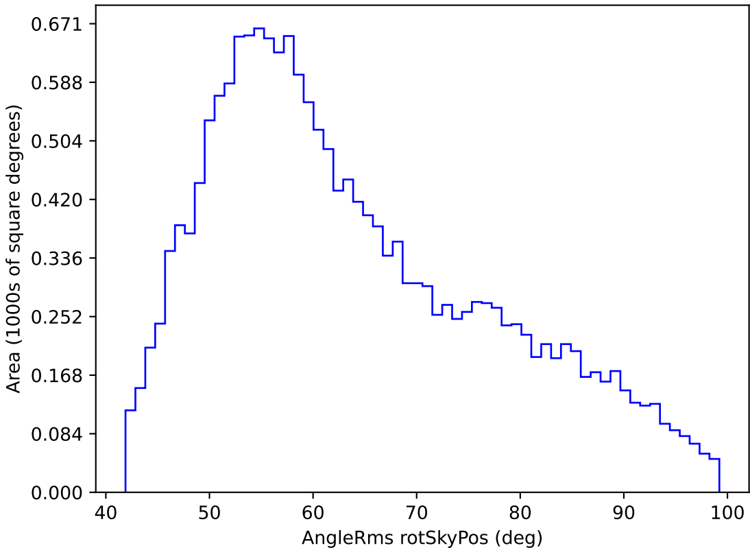
weather_cloudso35v3.4_10yrs WFD u band: AngleRms rotSkyPos
