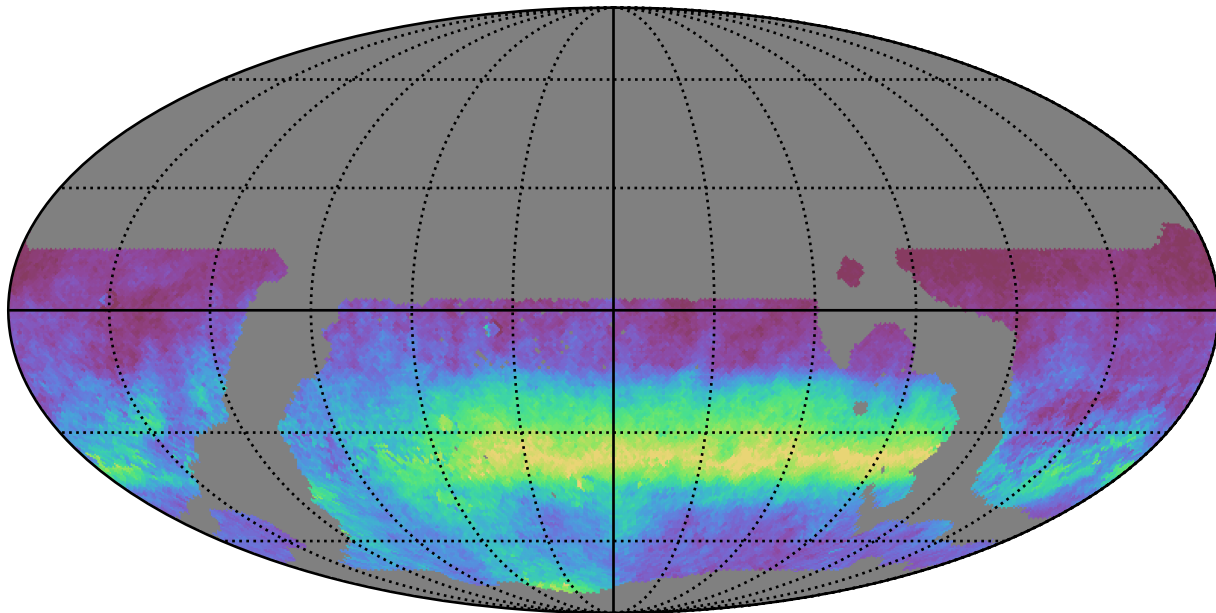
weather_cloudso35v3.4_10yrs WFD r band: AngleRms rotSkyPos
