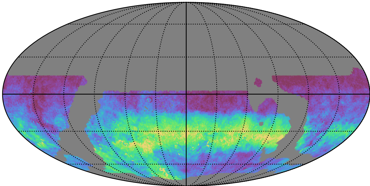
weather_cloudso35v3.4_10yrs WFD g band: AngleRms rotSkyPos
