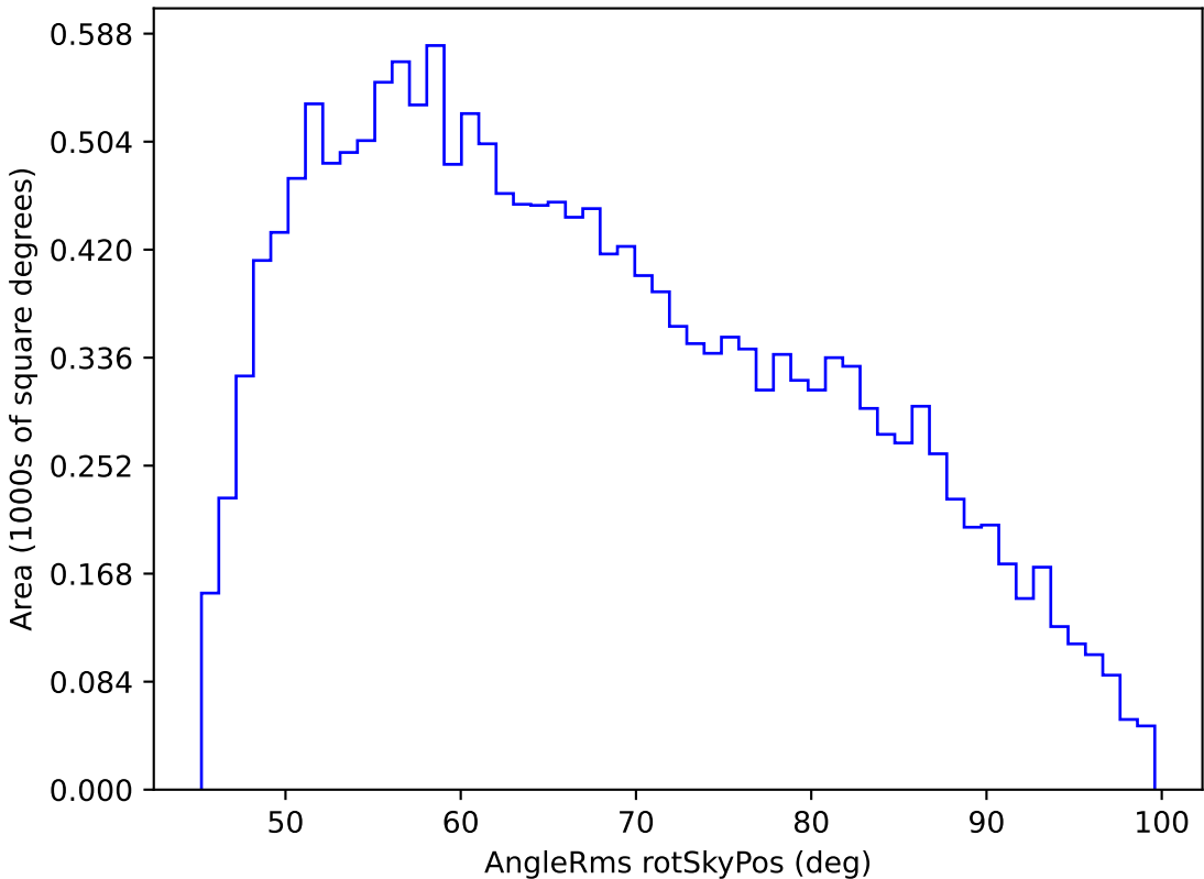
weather_cloudso35v3.4_10yrs WFD g band: AngleRms rotSkyPos
