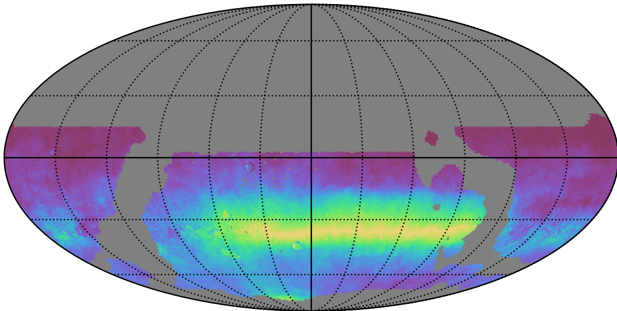
weather_cloudso35v3.4_10yrs WFD all bands: AngleRms rotSkyPos
