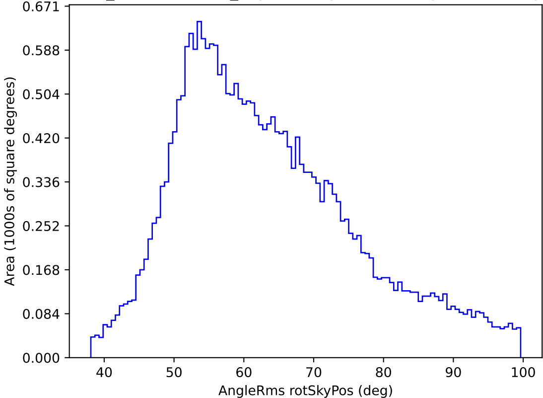
weather_cloudso35v3.4_10yrs All sky z band: AngleRms rotSkyPos
