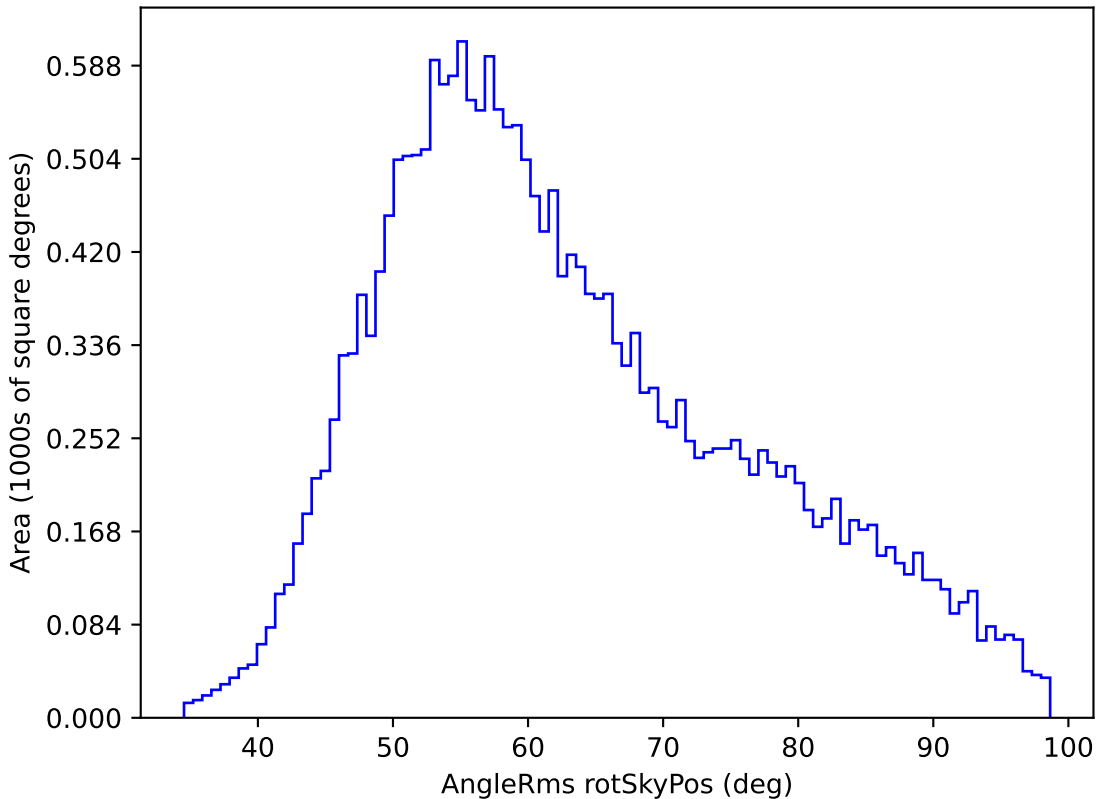
weather_cloudso35v3.4_10yrs All sky u band: AngleRms rotSkyPos
