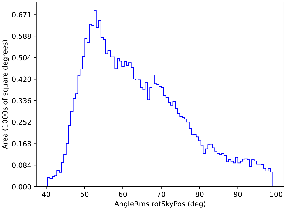
weather_cloudso35v3.4_10yrs All sky r band: AngleRms rotSkyPos
