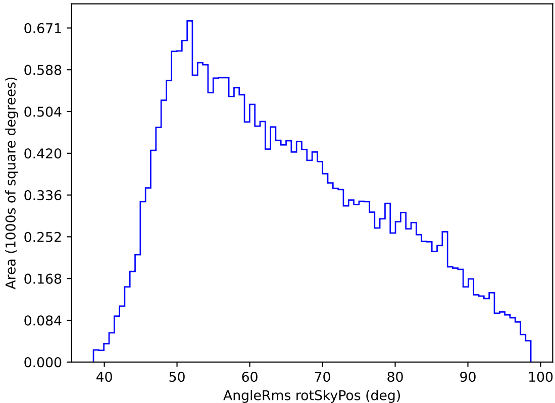
weather_cloudso35v3.4_10yrs All sky g band: AngleRms rotSkyPos
