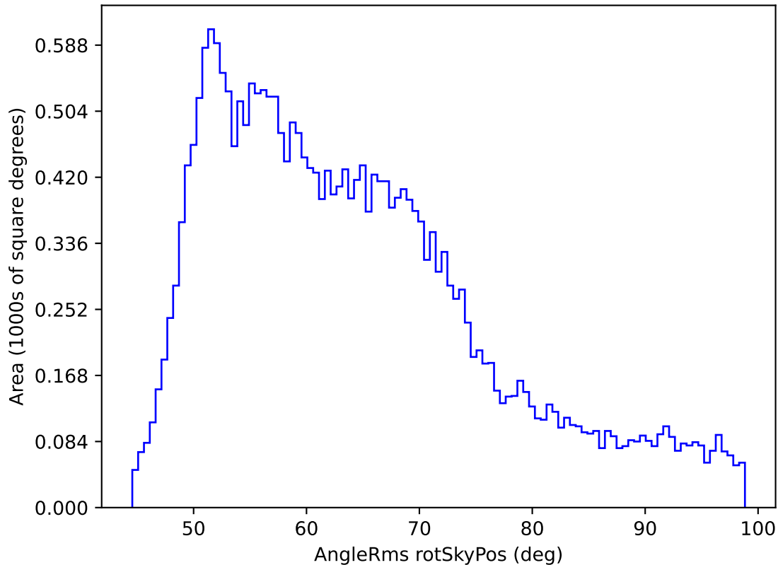
weather_cloudso35v3.4_10yrs All sky all bands: AngleRms rotSkyPos
