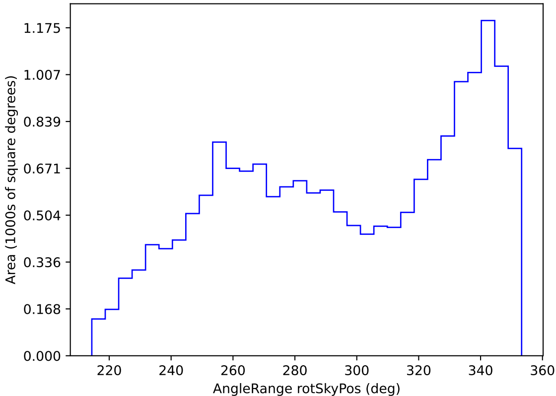
weather_cloudso35v3.4_10yrs WFD all bands: AngleRange rotSkyPos
