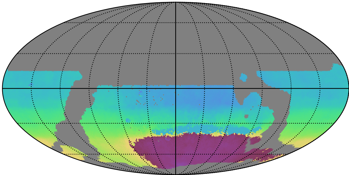
weather_cloudso35v3.4_10yrs WFD all bands: AngleMean rotSkyPos
