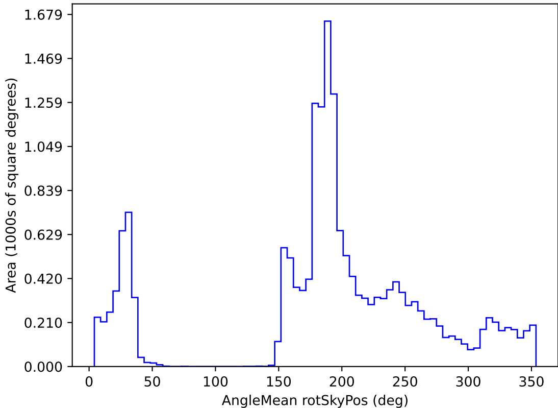
weather_cloudso35v3.4_10yrs WFD all bands: AngleMean rotSkyPos
