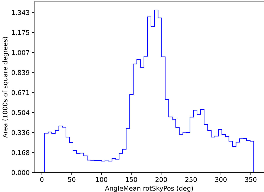
weather_cloudso35v3.4_10yrs All sky u band: AngleMean rotSkyPos
