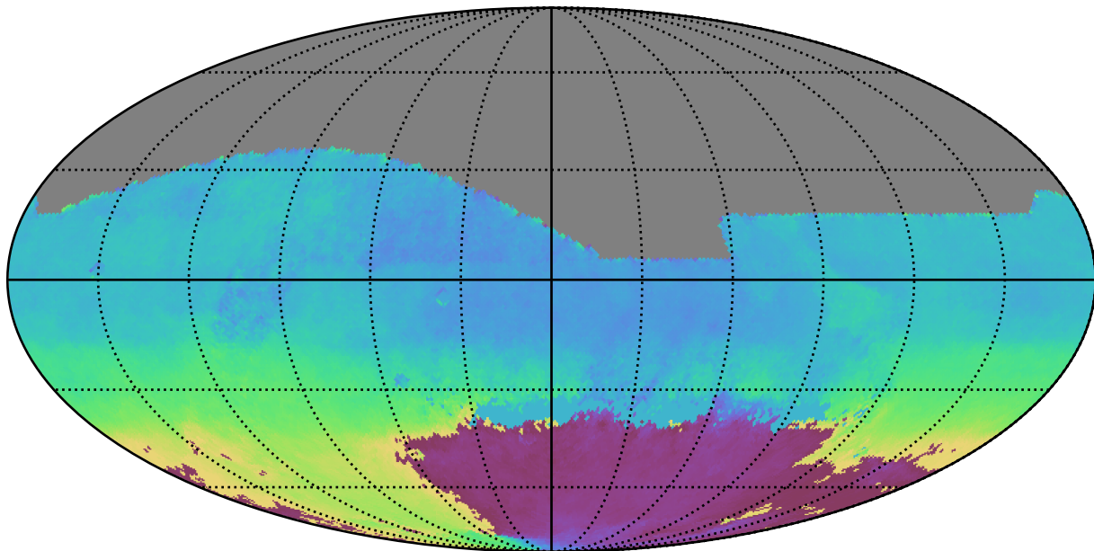
weather_cloudso35v3.4_10yrs All sky r band: AngleMean rotSkyPos
