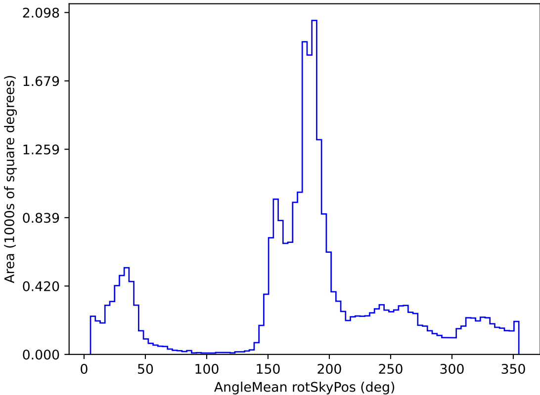
weather_cloudso35v3.4_10yrs All sky r band: AngleMean rotSkyPos
