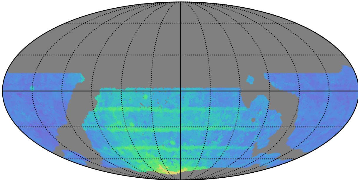
weather_cloudso35v3.4_10yrs WFD z band: 80thPercentile Season Length
