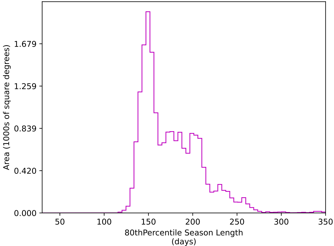
weather_cloudso35v3.4_10yrs WFD z band: 80thPercentile Season Length
