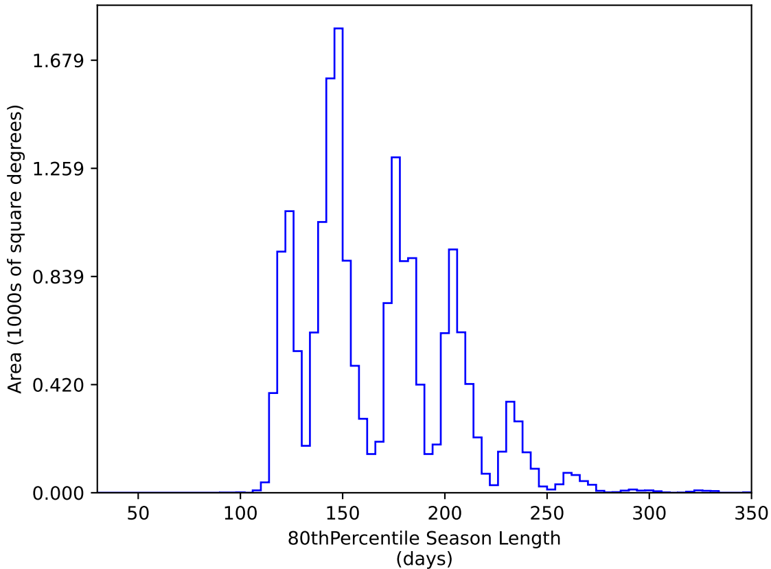
weather_cloudso35v3.4_10yrs WFD y band: 80thPercentile Season Length
