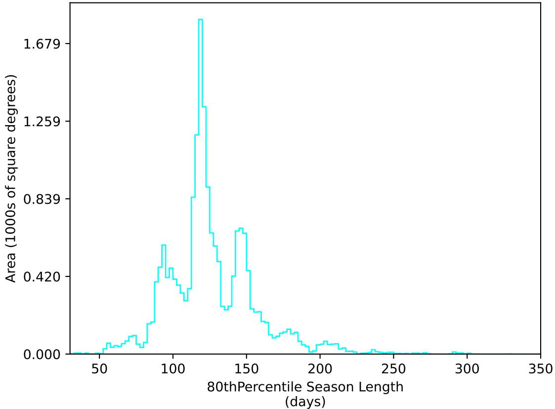
weather_cloudso35v3.4_10yrs WFD u band: 80thPercentile Season Length
