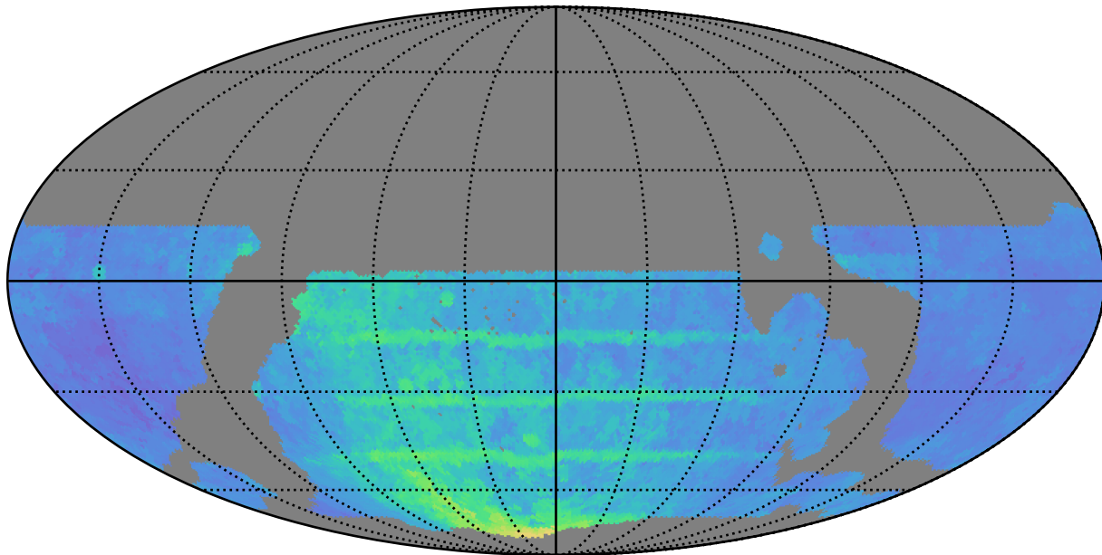
weather_cloudso35v3.4_10yrs WFD r band: 80thPercentile Season Length
