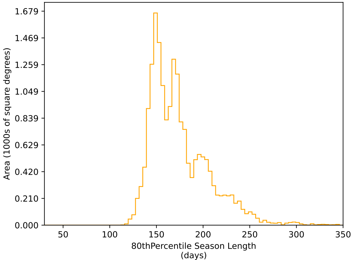
weather_cloudso35v3.4_10yrs WFD r band: 80thPercentile Season Length
