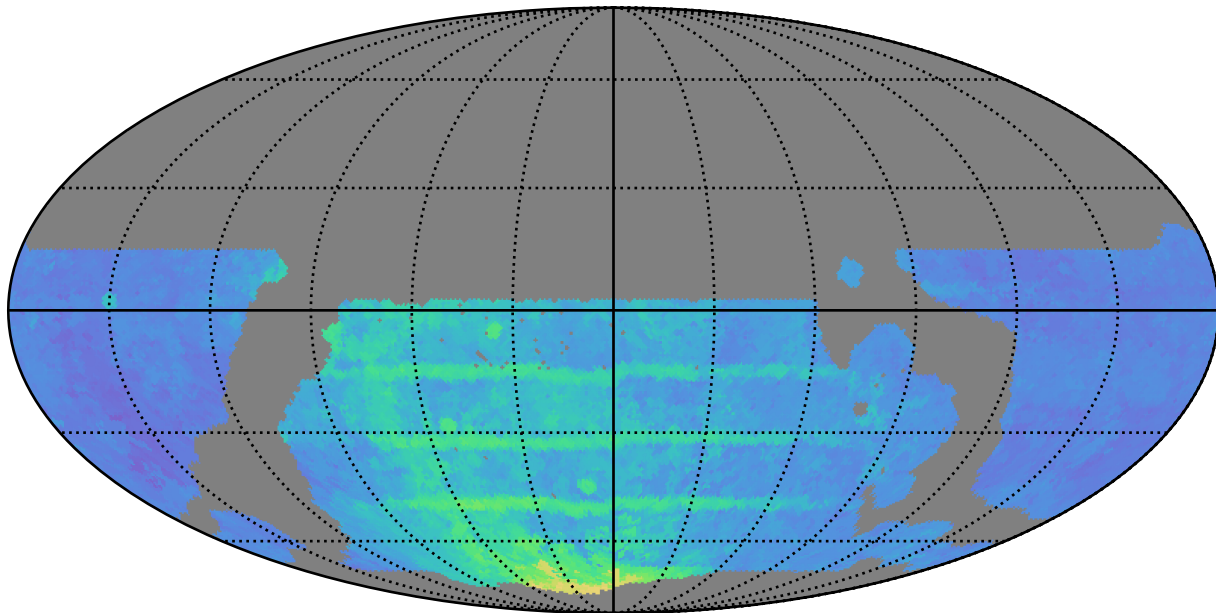
weather_cloudso35v3.4_10yrs WFD i band: 80thPercentile Season Length
